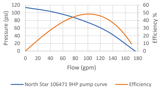
North Star 106471 9HP pump curve
