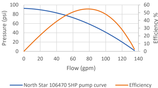
North Star 106470 5HP pump curve
